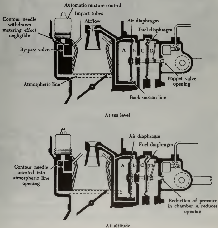
FIGURE 3-25. Automatic mixture control system.
